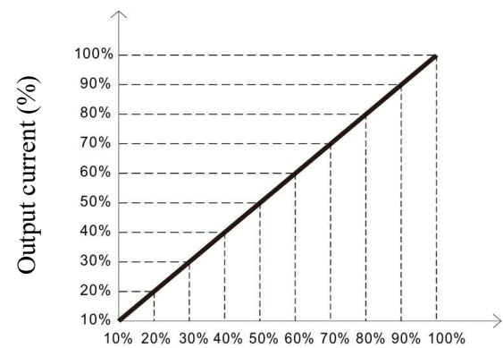
Duty cycle of additive 10V PWM signal dimming
